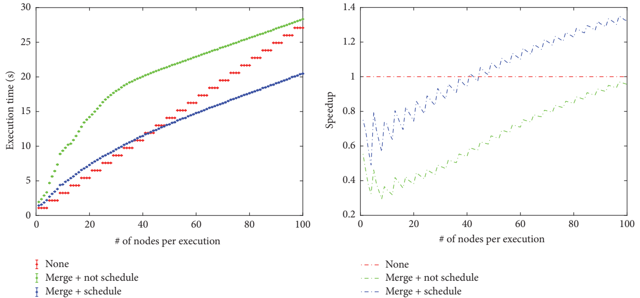
FIGURE 13: Average execution time and speedup for different strategies.
