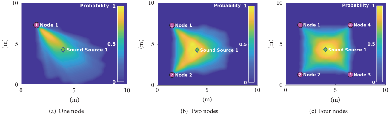
FIGURE 5: Our data fusion technique combines the polar steering response map produced by each node to generate a probability map that estimates the location of the observed sound sources. As more nodes are used, the localization accuracy is improved. This technique has been adapted from [1].
