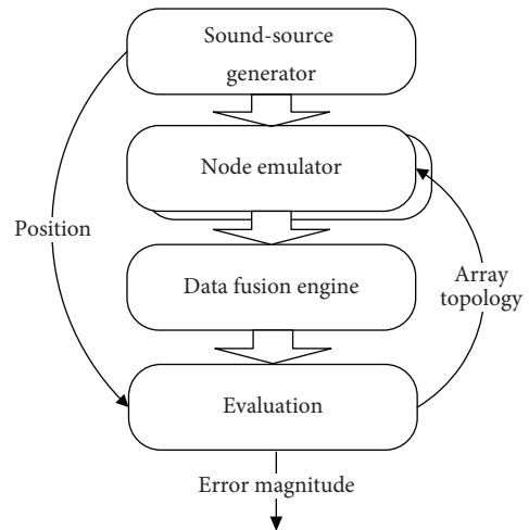
FIGURE 3: Execution steps of the NE. The sound sources are generated and processed by the nodes. The nodes of the network are reconfigured based on the error obtained after the evaluation of the data fusion.
