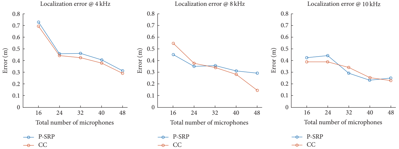
FIGURE 11: The localization error, using one sound source and four nodes at three different frequencies, improved as the total number of microphones in the network increased. Both methods, P-SRP and CC, performed equivalently.
