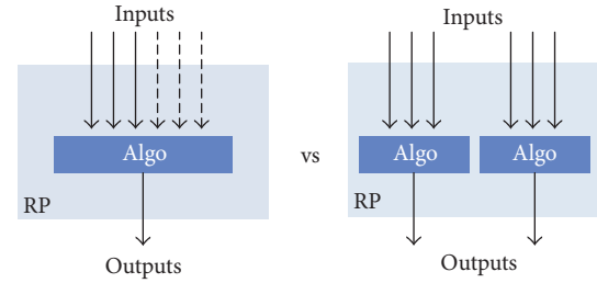
FIGURE 1: The use of PR allows us to exploit the available resources for different algorithm's configurations. For instance, when not all the input data need to be processed (dash arrows) the RP can be reconfigured to allocate more instances of the algorithm, doubling the throughput in this example.
