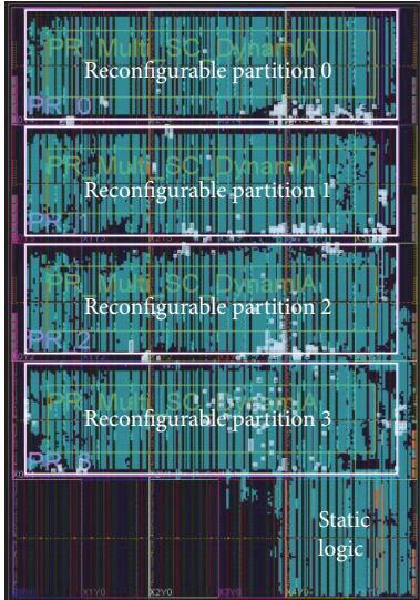
FIGURE 9: FPGA floorplanning when all nodes have their subarrays active. The four reconfigurable partitions of the NE are framed into white boxes.
