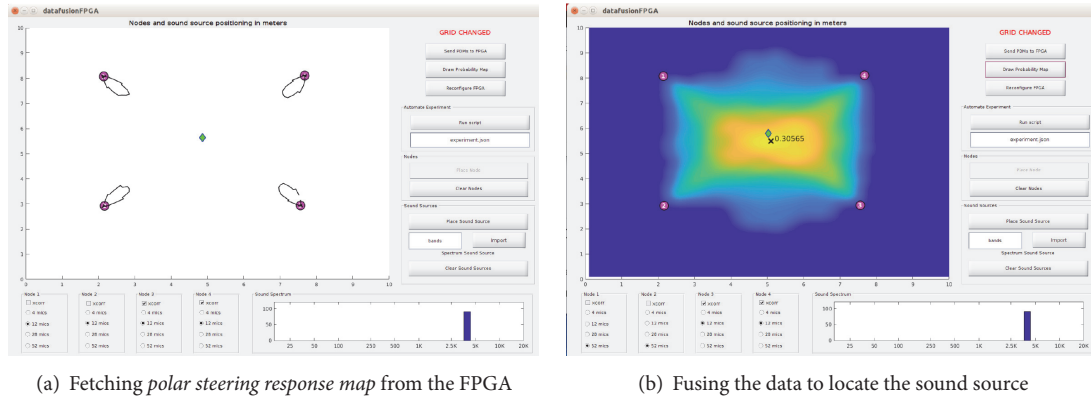
FIGURE 4: The data fusion front-end is capable of simulating a sound field with multiple sound sources (green diamond) and multiple nodes (pink circles). The front-end generates PDM signals for each microphone in each node that are then sent to the FPGA back-end. The FPGA generates the corresponding polar steering response map (a) which is then fed to the data fusion algorithm to generate a probability map (b) and estimate the localization error.
