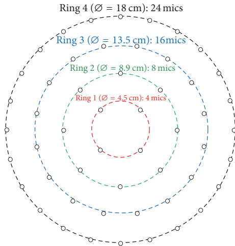
FIGURE 7: Sound source localization device composed of 4 digital MEMS microphone subarrays.
