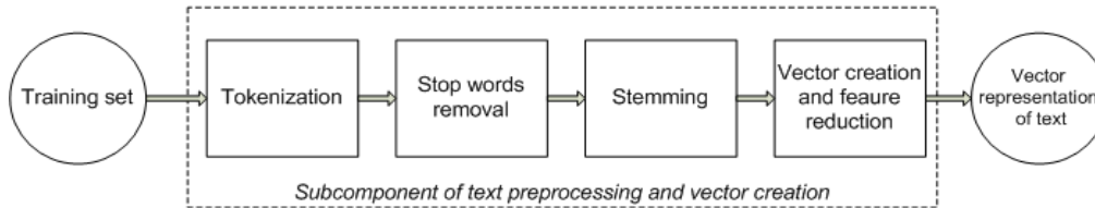
Figure 2: Schema of the structure of the subcomponent of text preprocessing and vector creation
